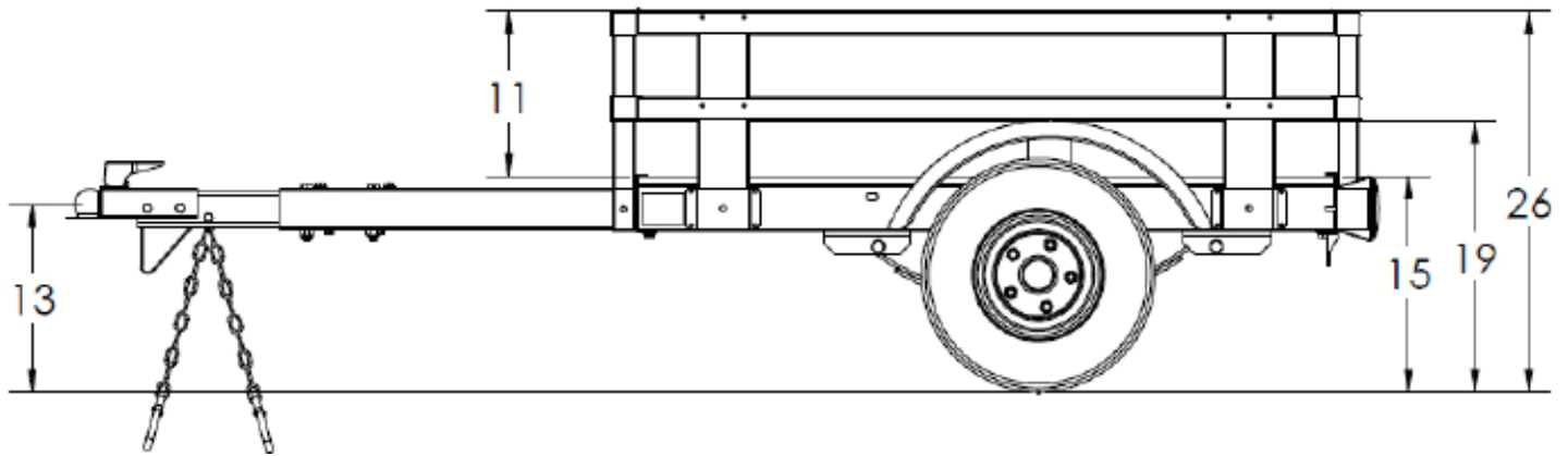
Side View
