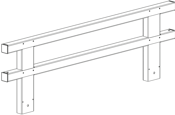
4X4 KIT TRAILER - 15" RAIL SIDE (504685)
