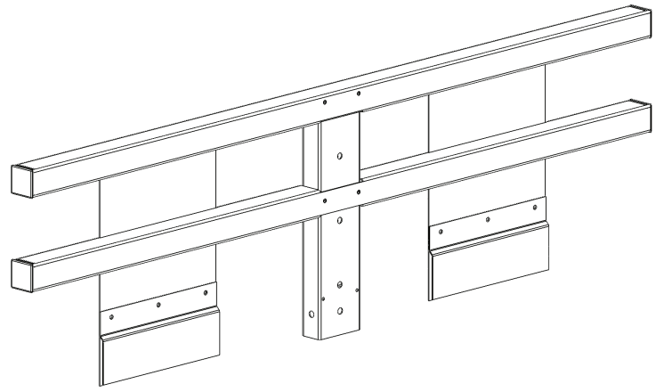
4' - 15" REAR RAMP RAIL SIDE (504662)
