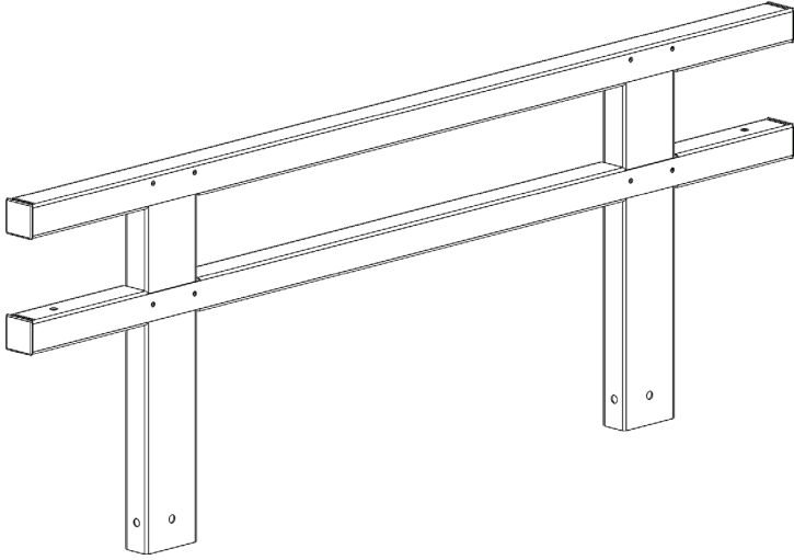
4' - 19" FRONT/REAR RAIL SIDE (504718)
