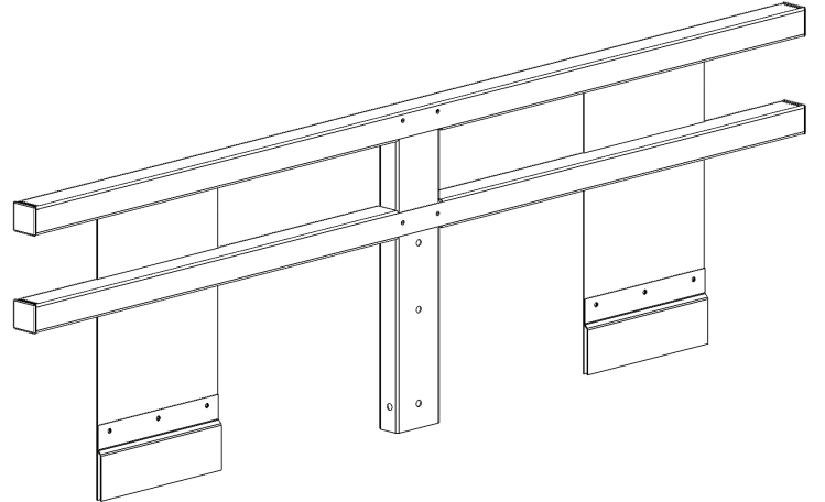
5' - 19" REAR RAMP RAIL SIDE (504693)
