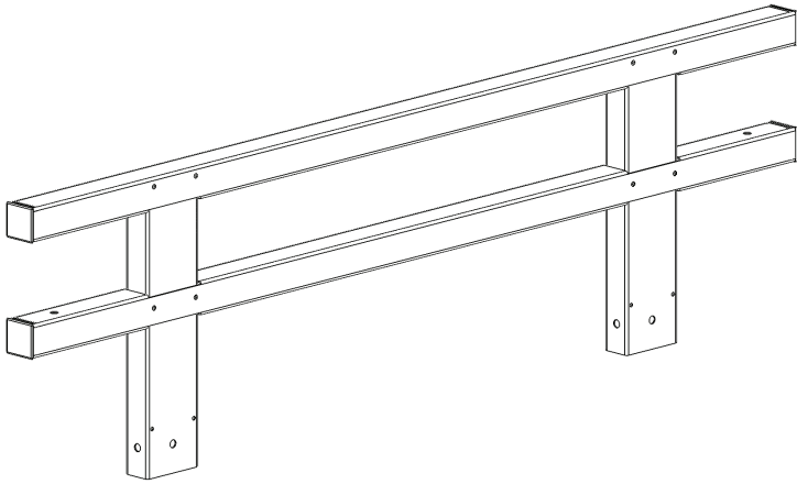
4' - 15" FRONT/REAR RAIL SIDE (504659)
