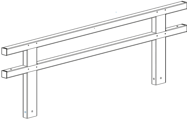
5' - 19" FRONT/REAR RAIL SIDE (504690)
