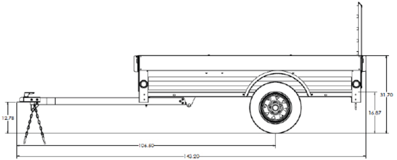
Side View
